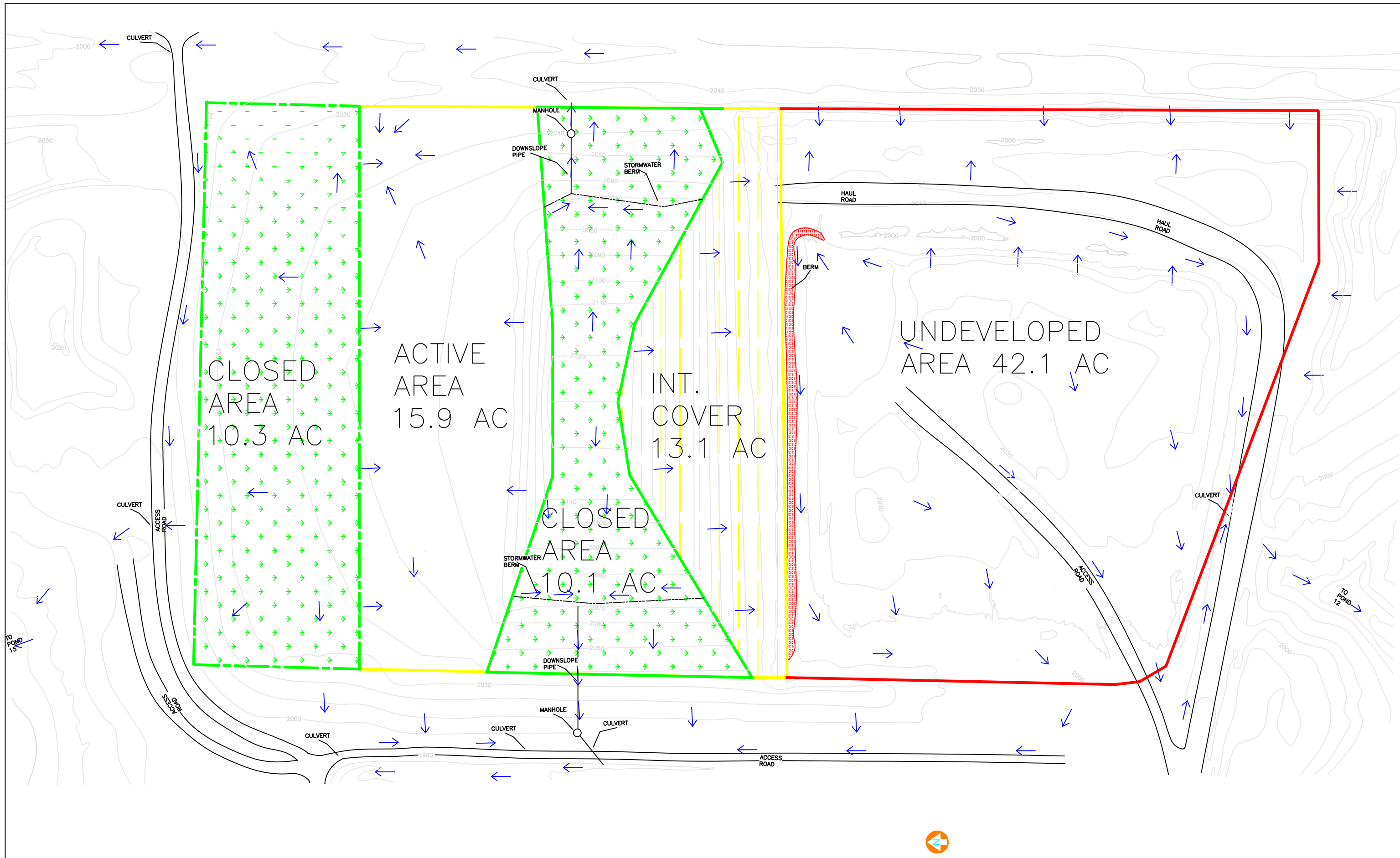
FIGURE 1 BLUE PIT DRAINAGE MAP
